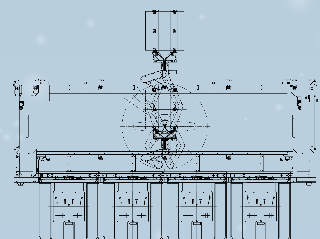
4 Port Panel Transfer EFEM
